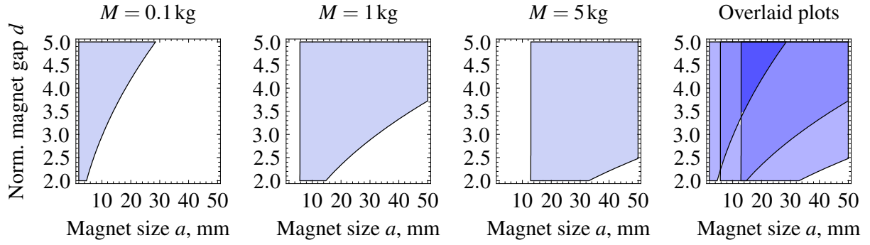
Fig. 7. Regions of a and d satisfying the static deflection criterion of equation (21) for a range of masses. Darker sections denote overlap of the regions in the overlay plot.
