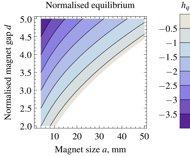
Fig. 5. Map of the normalised equilibrium position over varying magnet size a and normalised magnet gap d for a system with mass M = 0.5 kg.
