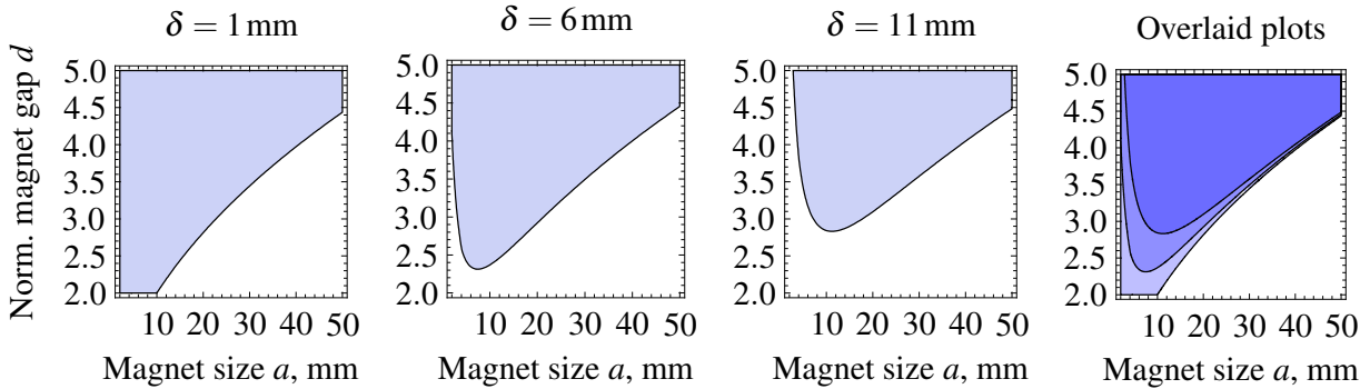
Fig. 11. Region of a, d satisfying the stability criterion of equation (24) for a range of disturbance displacements \delta and a normalised displacement tolerance \epsilon = 0.1 . Darker sections denote overlap of the regions in the overlay plot.
