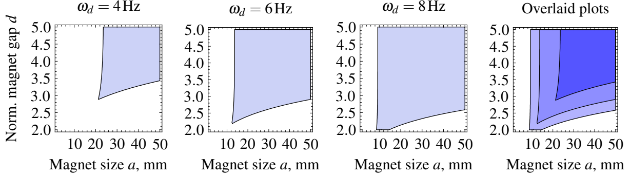
Fig. 8. Regions of a and d satisfying the resonance frequency criterion of equation (22) for a range of allowable resonance frequencies and a mass M = 0.5 kg. Darker sections denote overlap of the regions in the overlay plot.
