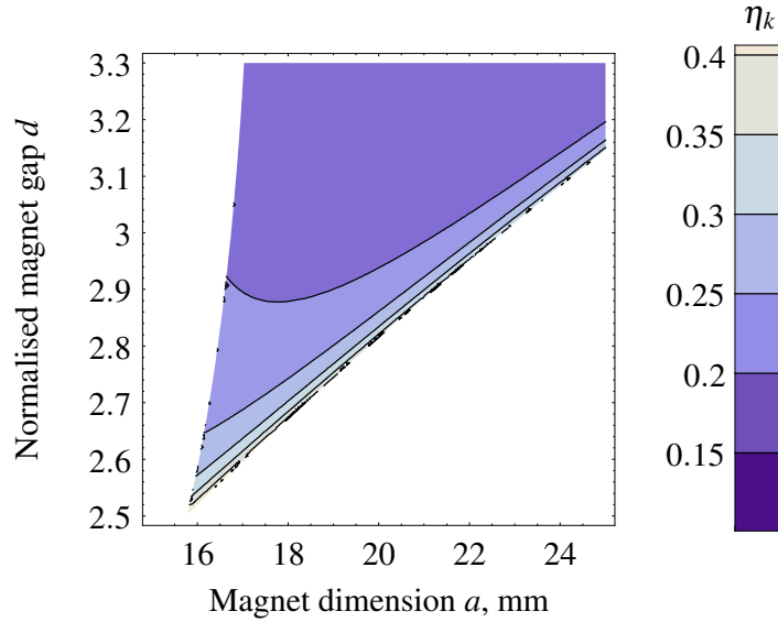
Fig. 15. Zoom of Figure 14 to show the behaviour of the nonlinearity in the lower limits of the magnetic spring.
