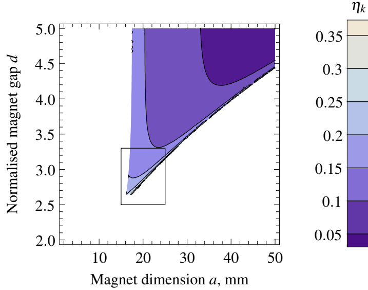
Fig. 14. Contours of nonlinearity shown inside the region of a, h satisfying all criteria for parameters M = 1\text{ kg} , \omega_d = 5\text{ Hz} , \delta = 1\text{ mm} , \varepsilon = 0.1 . A closeup (of the box) is shown in Figure 15.
