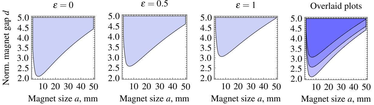
Fig. 10. Regions of a and d satisfying the the stability criterion of equation (24) for a range of normalised displacement tolerances \epsilon and a maximum disturbance displacement of \delta = 5\text{mm} . Darker sections denote overlap of the regions in the overlay plot.
