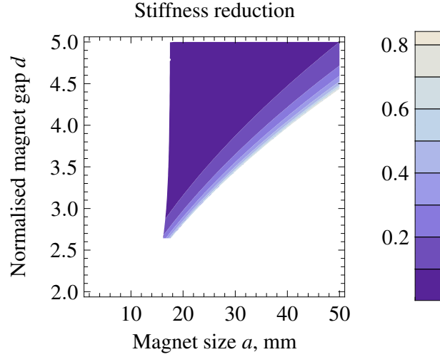
Fig. 13. Contours of stiffness reduction \kappa due to the negative stiffness of the attractive magnet, shown inside the region of a, d satisfying all design criteria for parameters M = 1 kg, \omega_d = 5 Hz, \delta = 1 mm, \varepsilon = 0.1 .
